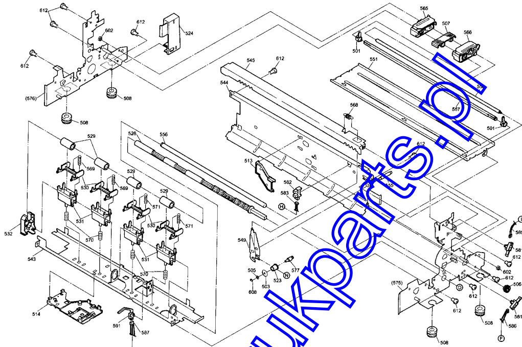
EXPLODED DIAGRAM FOR LQ-670 (3/3)
