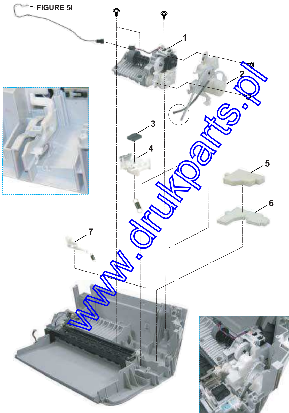
FIGURE 9 SEPARATION UNIT
