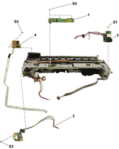
FIGURE 9 CARRIAGE UNIT & PURGE UNIT
